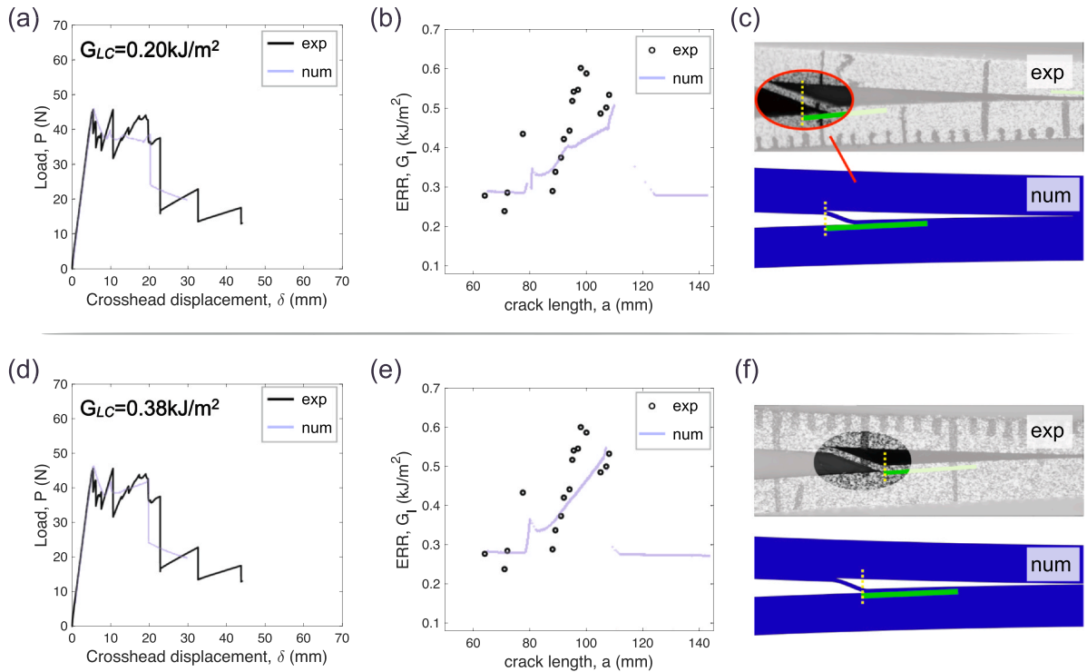
Fig. 6. Comparison between experimental responses and numerical results using two cohesive fracture toughness values of the arrest region. The selected toughness values are the lowest and the highest values obtained from uniform LC, (a) Load–displacement curves, (b) corresponding R-curves, and (c) local damage observations of 0.20 kJ/m 2 , while (d) load–displacement curves, (e) corresponding R-curves, and (f) local damage observations of 0.38 kJ/m 2 . Dashed yellow lines in (c) and (f) highlight the beginning of the arrest regions, which are illustrated in green.
