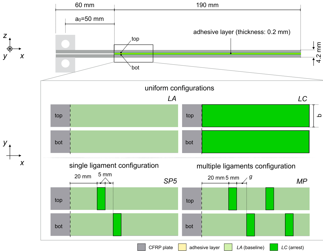
Fig. 1. Schematics of investigated surface pretreatments. The DCB specimen has a width b = 20 mm. Two uniformly treated surfaces LA and LC . The single patterning of LA and LC , denoted as SP5 , has the anchor size and gap distance equal to 5 mm. Three different multiple patterns are obtained by changing the gap distance g between the adjacent arrest treatments. MP2 , MP5 , and MP10 stand for gap distance of 2.5, 5, and 10 mm, respectively.
