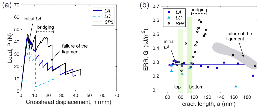
Fig. 2. Typical load–displacement curve and the corresponding ERR of single patterning SP5. Typical global responses of uniform LA and LC are also illustrated for comparison. The dashed lines indicate the regimes with the bridging of adhesive ligaments. The arrest LC region is highlighted in green in the R-curve.
