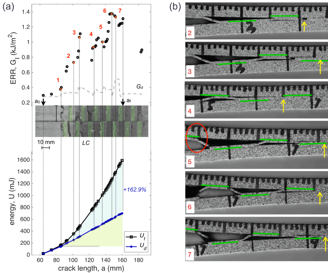
Fig. 5. (a) R-curve, nominal detachment ERR G_d , fracture surface, and integrated energy evolution U_i of MP2. (b) In situ corresponding crack propagation observed from the side of the DCB specimen. The arrest regions LC are highlighted in green and yellow arrows indicate positions of the crack tip.
