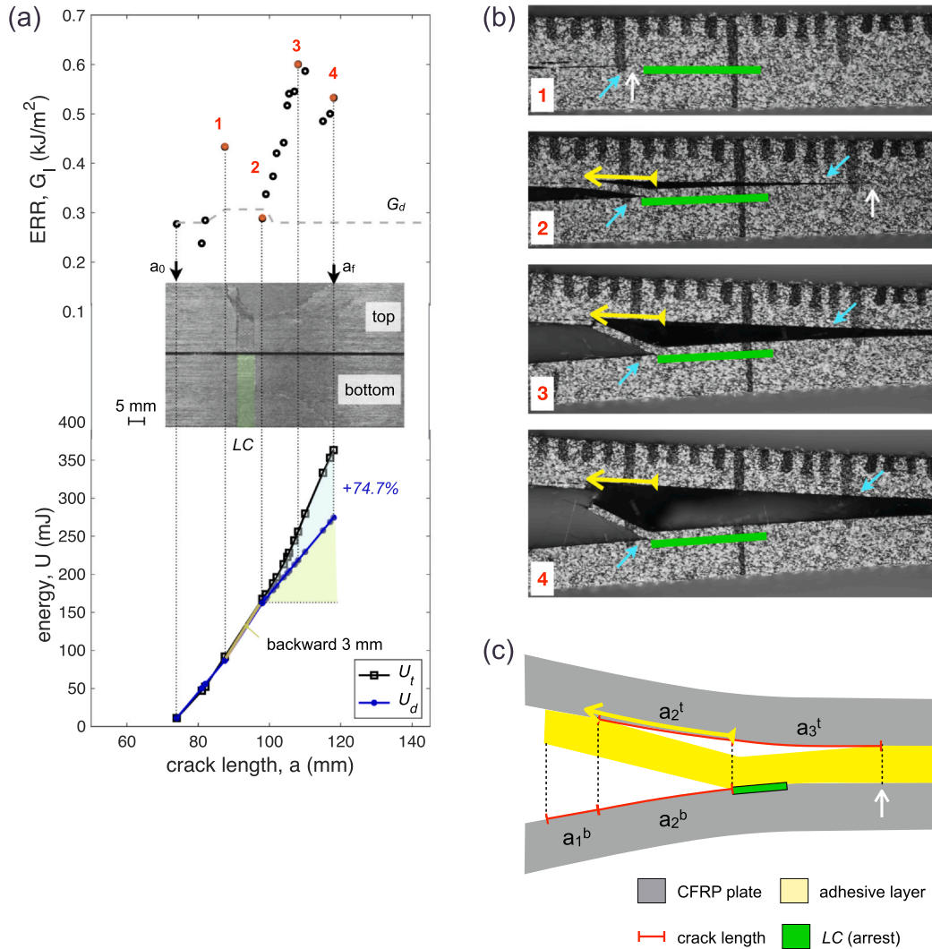
Fig. 3. (a) R-curve, nominal detachment ERR G_d , fracture surface, and integrated energy evolution U_t of SP5. The backward crack length is highlighted between point 1 and 2. (b) In situ corresponding crack propagation observed from the side of the DCB specimen. Upward cyan arrows indicate the primary crack, while downward cyan arrows point to the secondary crack on the top CFRP/adhesive interface. The backward crack propagation areas are illustrated in yellow and the arrest regions LC are highlighted in green. White arrows point to the location of the crack tip. (c) Schematic of the decomposition of the crack length.
