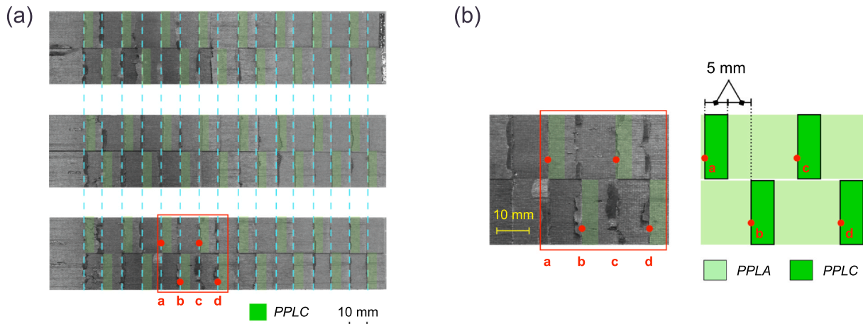
Fig. 8. (a) Fracture surfaces of DCB specimens with PPLA/PPLC patterning. Dash cyan lines highlight the breakage location of the adhesive layer. The arrest regions PPLC are highlighted in green. (b) Zoomed fracture surface in the red box and corresponding schematic of the surface patterning in the chosen region.
