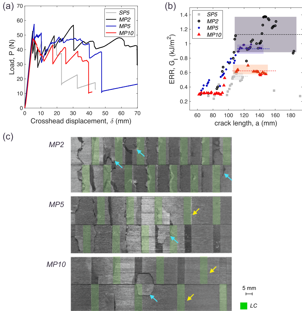
Fig. 4. (a) Typical load–displacement curve and (b) the corresponding ERR of multiple patterning MP2, MP5, and MP10. Shaded areas highlight the stabilization stage and dashed lines indicate the average ERR within this stage. Typical global responses of SP5 are also illustrated for comparison. (c) Fracture surfaces of multiple patterning MP2, MP5, and MP10. Cyan arrows point to the partial adhesive ligaments and yellow arrows indicate the positions that failed to trigger ligaments.
